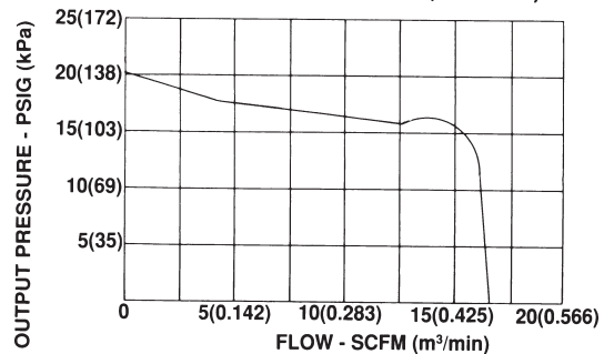
FLOW CHARACTERISTICS (TYPICAL)
